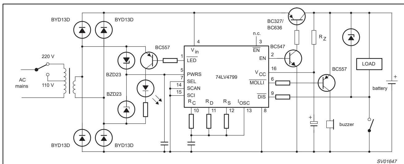
Figure 2. Typical application of the low-voltage 74LV4799.
