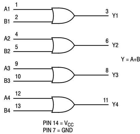
LOGIC DIAGRAM
