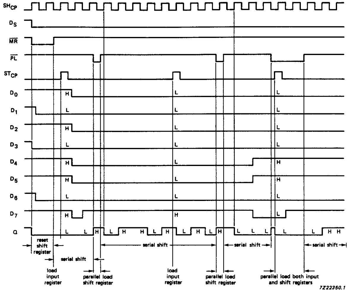
Fig.6 Timing diagram.
