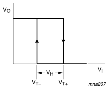
Fig 8. Transfer characteristics
