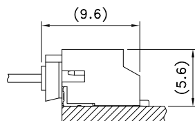
RECOMMENDED ASSEMBLY DIM.
