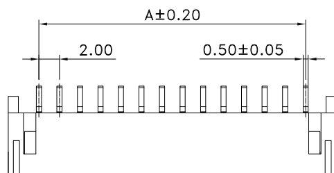
RECOMMENDED PCB LAYOUT DIM. General tolerance \pm 0.05
