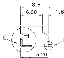
Detail E SCALE 4:1
