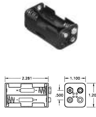
Holds Four (4) "AA" Cells in Series
