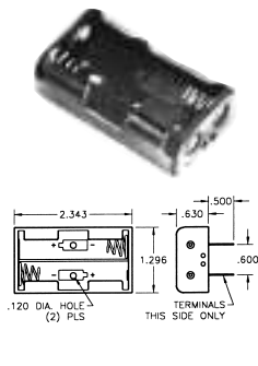
Holds Two (2) "AA" Cells in Series
