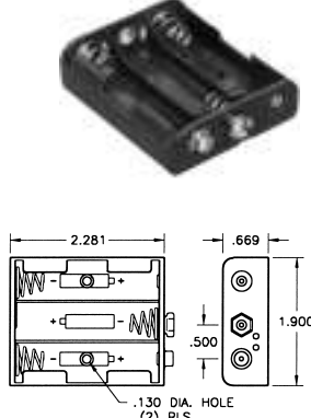
Holds Three (3) "AA" Cells in Series
