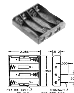
Holds Four (4) "AAA" Cells in Series
