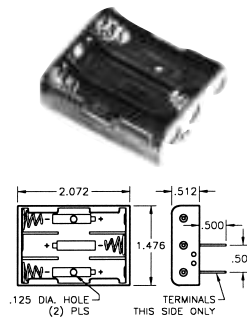
Holds Three (3) "AAA" Cells in Series
