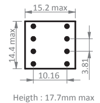
E 13 reinforced insulation creepage distances: 6mm
