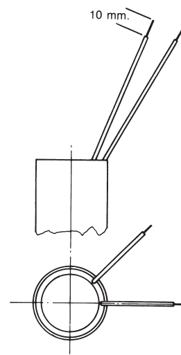
Fig. 5 Cavetti unipolari 0,5mm 2 L = 150 mm Fig. 5 Insulated solid core leads 0.5 mm 2 L = 150 mm
