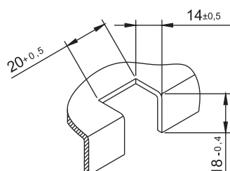
Mounting hole
