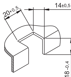
Mounting hole
