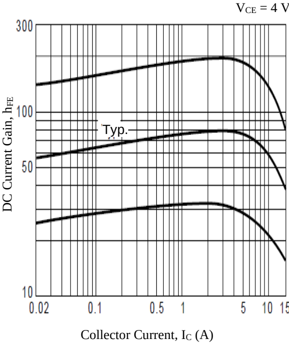
Figure 6. DC Current Gain Variation vs. Collector Current
