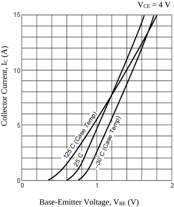
Figure 5. Collector Current vs. Base-Emitter Voltage
