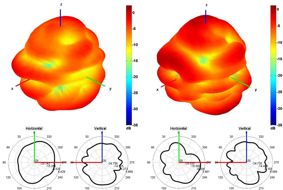
Cable 2: CELLULAR/LTE
