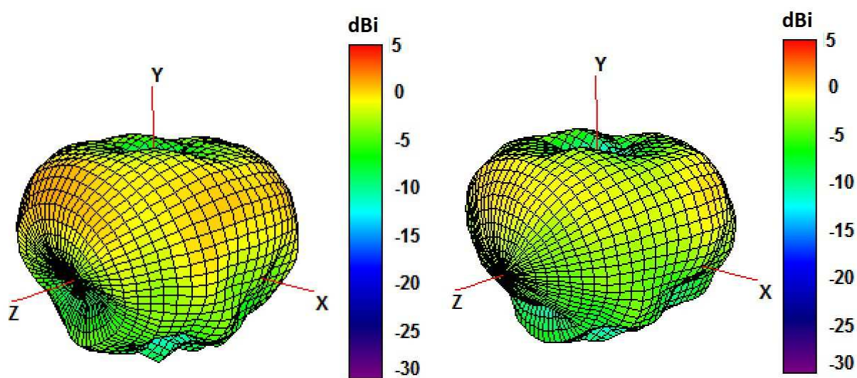
1750 and 1850 MHz Radiation pattern
