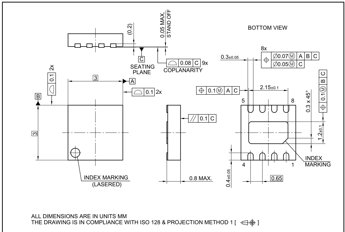
Figure 30 PG-WSO8-8 outline
