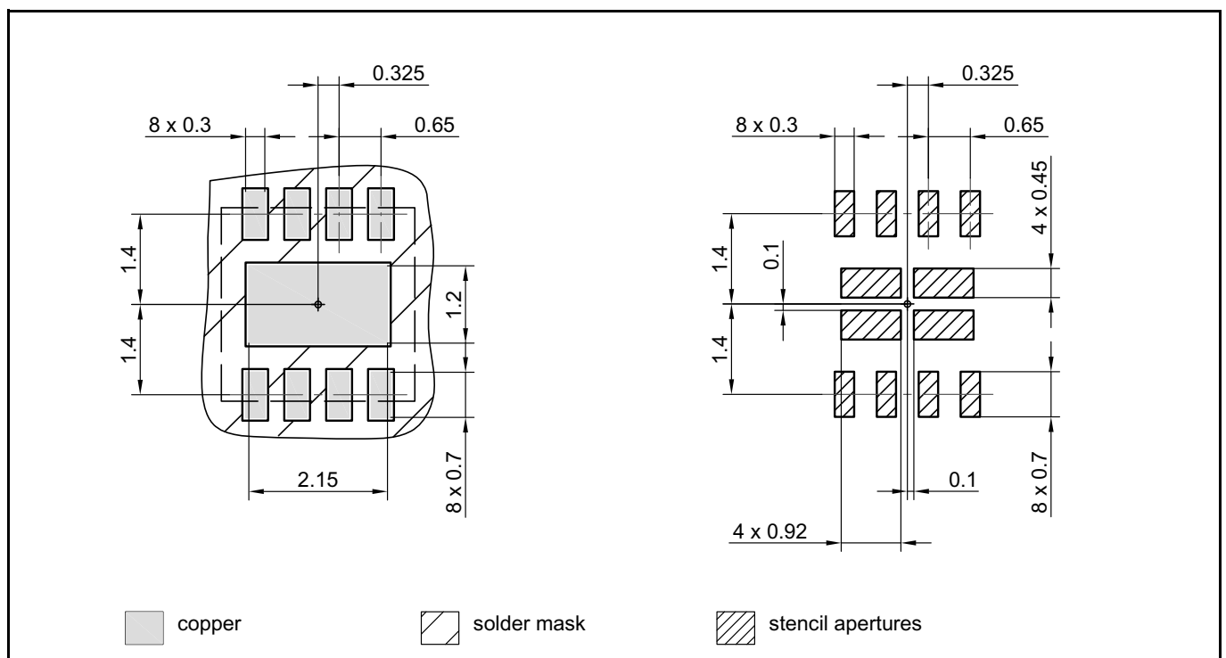
Figure 31 PG-WSO8-8 footprint
