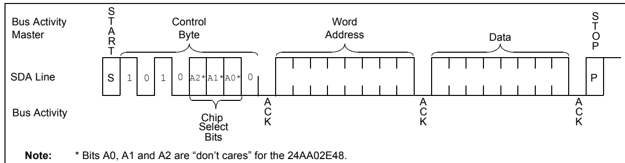
FIGURE 6-1: BYTE WRITE
