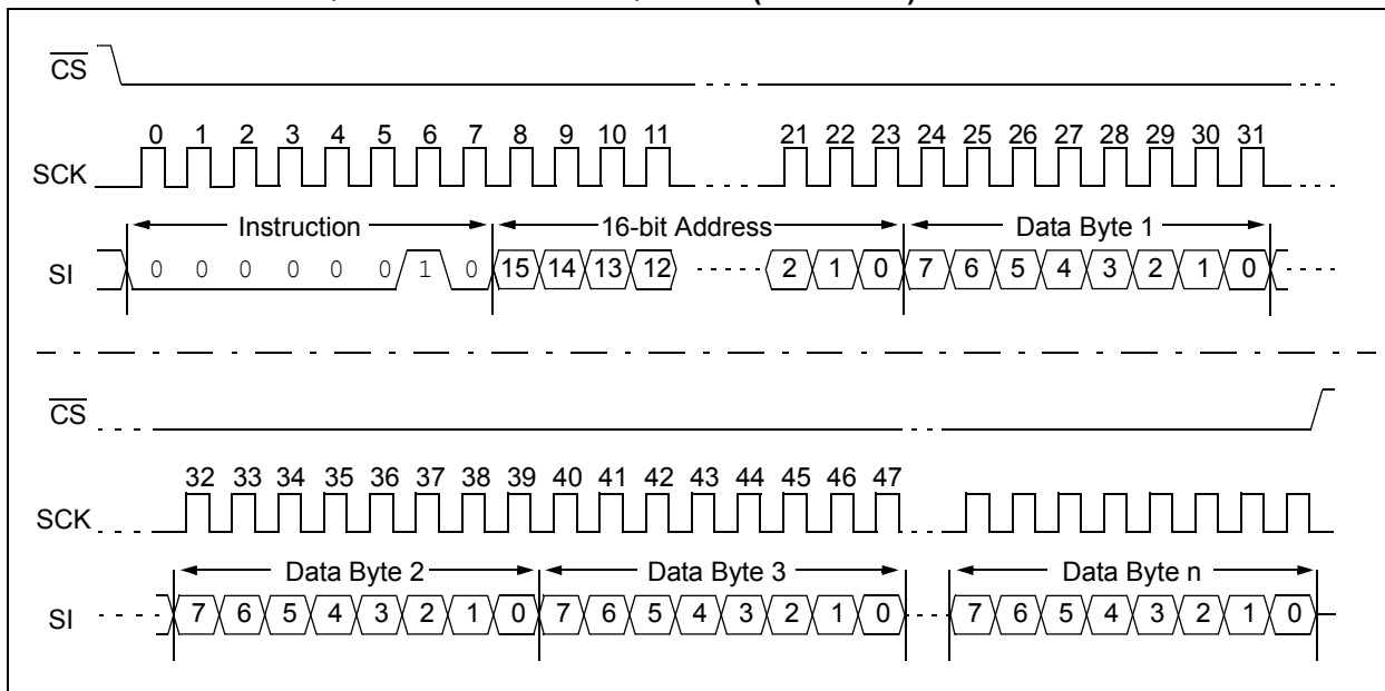
FIGURE 2-6: SEQUENTIAL WRITE SEQUENCE (SPI MODE)
