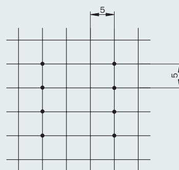
Soldering pin ø 0.6
