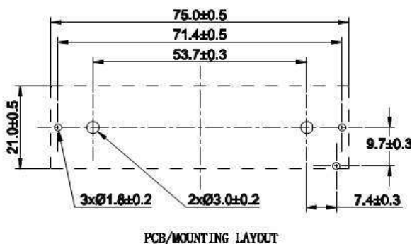
PCB/MOUNTING LAYOUT
