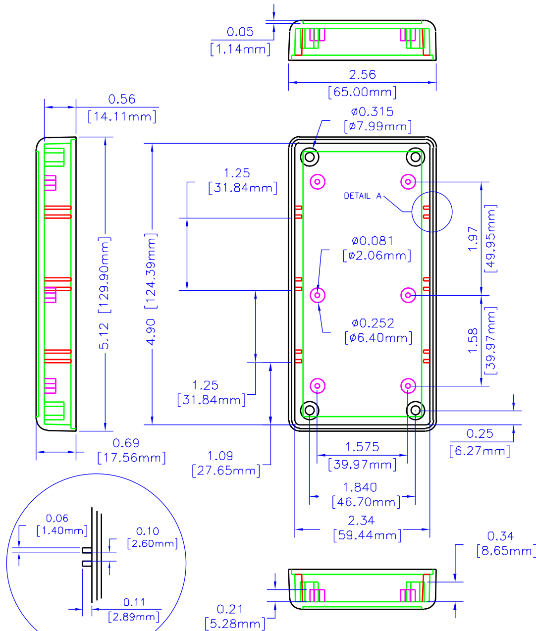
DETAIL A
