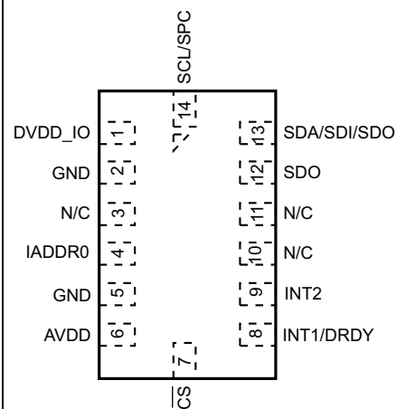
Figure 1. Pin Connections
